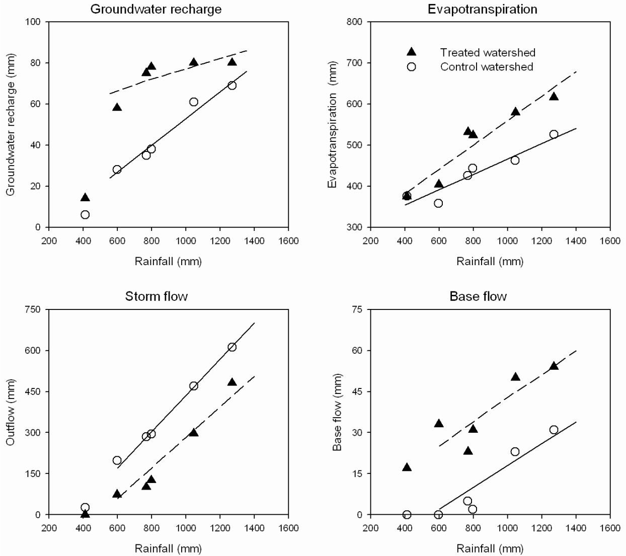
Figure 6: Impact of IWD intervention on i) groundwater recharge ii) ET iii) storm flow and iv) base flow generation. Open circles and triangles in figure presents control watershed and treated watershed, respectively (data from 2007 to 2012).
