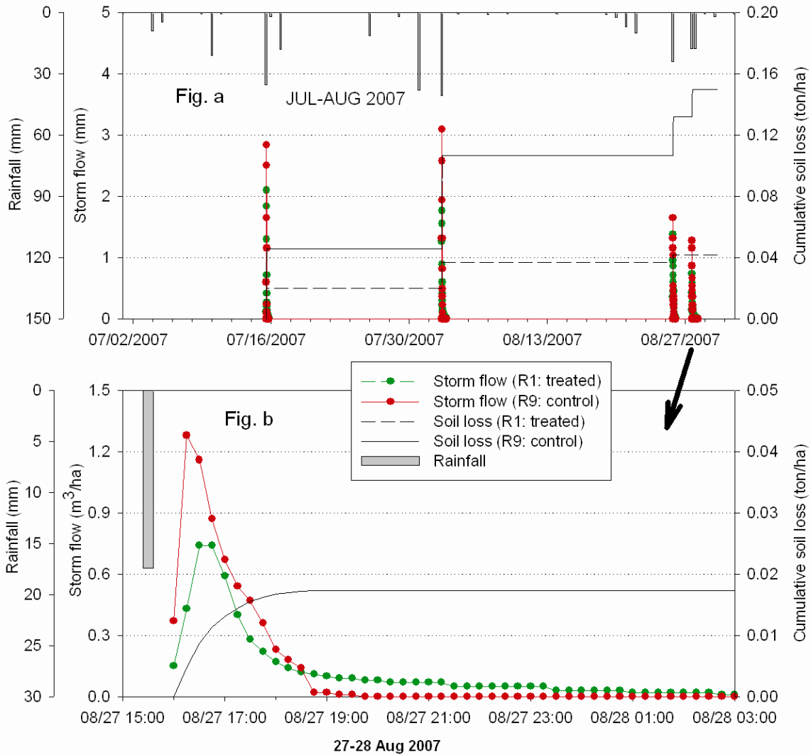
Figure 7 a) A comparison of storm flow and cumulative soil loss measured at reservoir-1 (R1) in treated watershed and R9 at control watershed in 2007; b) zoomed-in figure shows hydrograph and soil loss of selected event on 27-28 th Aug 2007 measured at R1 and R9
