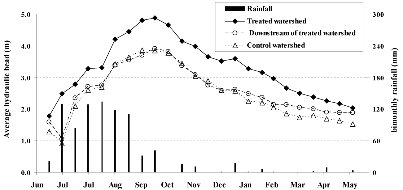
Figure 10a: Fluctuation of hydraulic head in relation to rainfall received on a fortnightly time scale in control, treated watershed and downstream villages of Garhkundar watershed.
