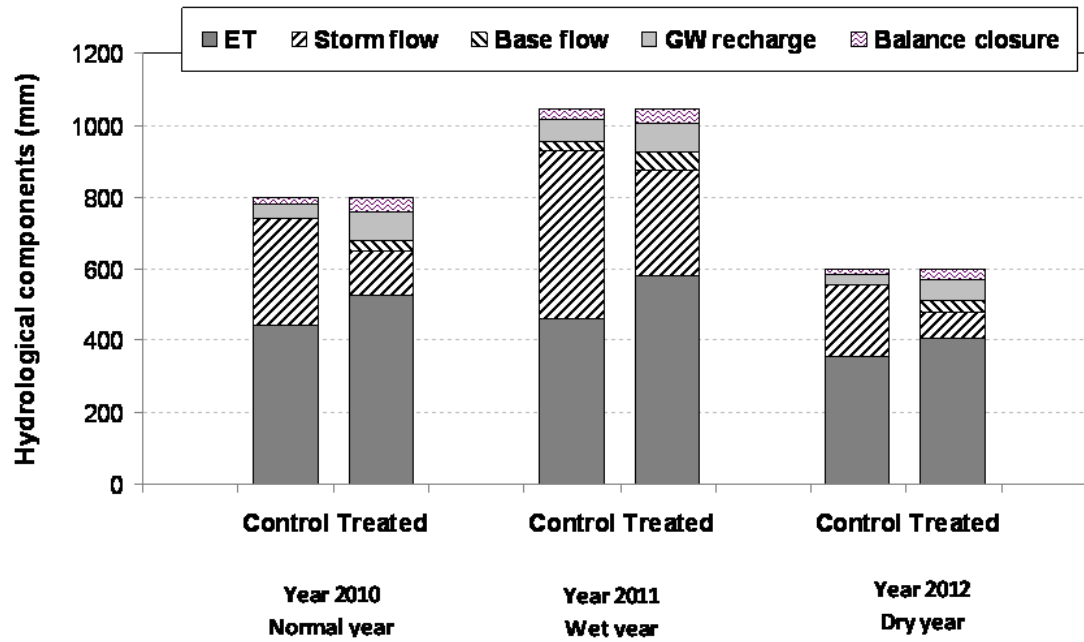
Figure 5: Water balance components (monsoonal) of selected normal, wet and dry years
