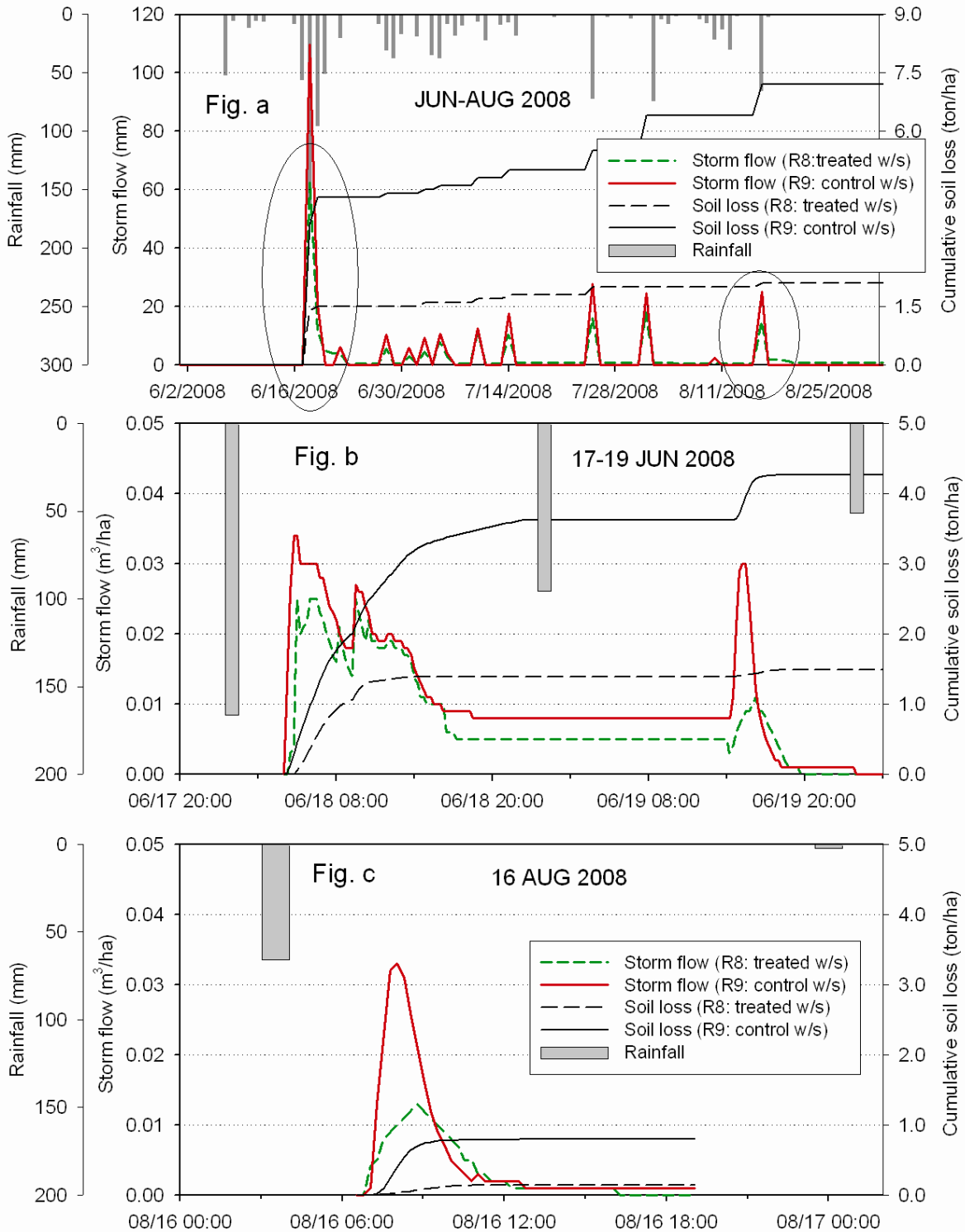
Figure 8 a) A comparison of storm flow and cumulative soil loss measured at outlet of treated watershed (R8) and control watershed (R9) in year 2008; b-c) zoomed-in figure (s) shows hydrograph and soil loss of selected events
