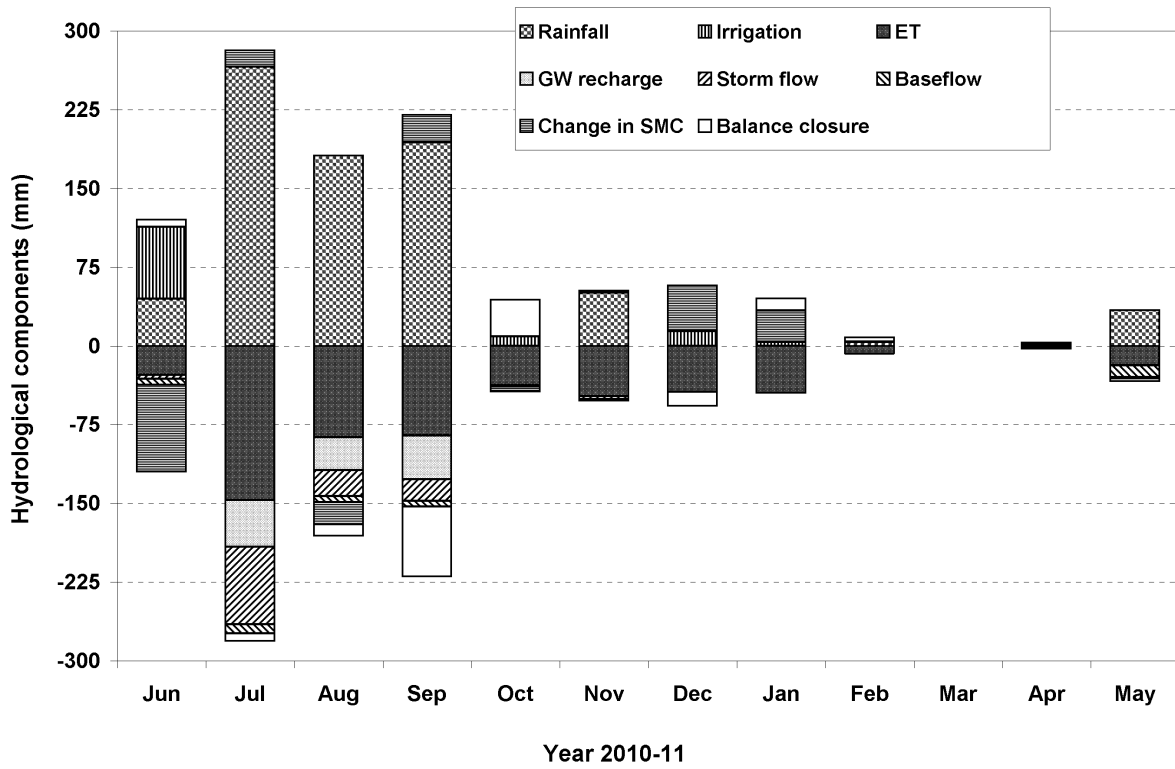
Figure 9: Month-wise water balance components of Garhkundar watershed (treated watershed) during year 2010-11
