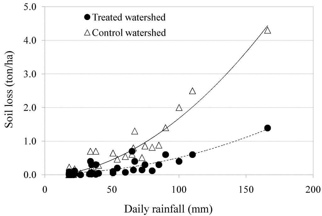
Figure 11: Rainfall intensity vs. rate of soil loss in treated and control watershed
