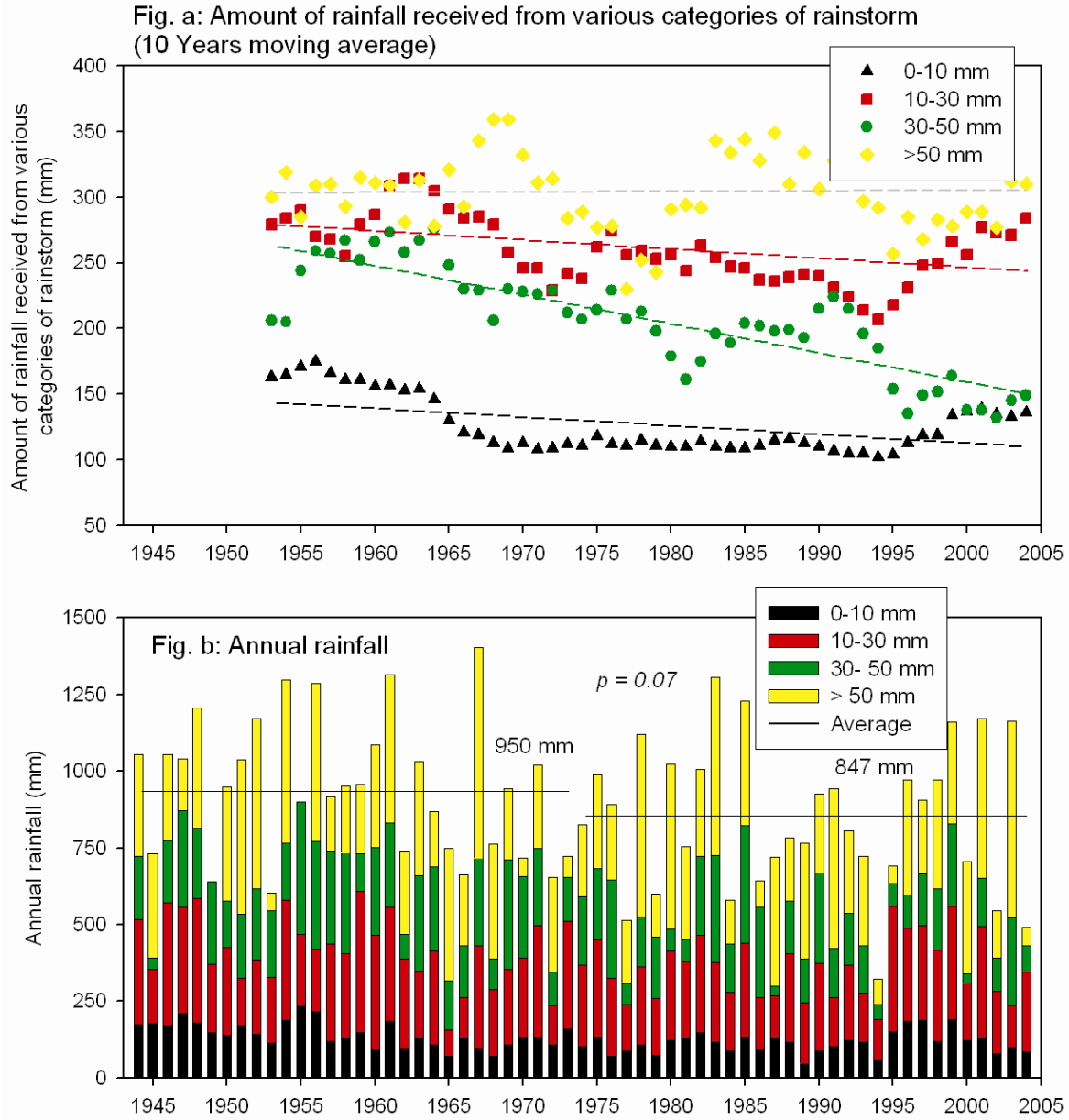
Figure 2 (a): Moving average (10 years) of rainfall received from various categories of rain events between 1945 and 2004; (b) Comparing annual rainfall between 1945-1974 and 1975-2004.
