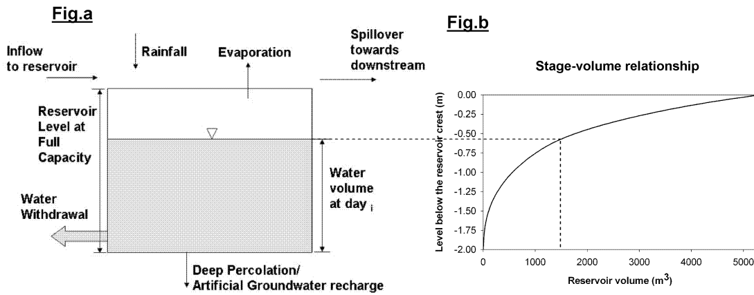
Figure 4: Schematic diagram of reservoir hydrology for small and medium storages structures. Reservoir water balance is defined as: Water volume at day i = Water volume at day i-1 + Inflow received (runoff) + Rainfall over the water body - Evaporation from the water body - Spillover amount – Infiltration from reservoir bottom (Artificial groundwater recharge)- Water withdrawn or utilized
