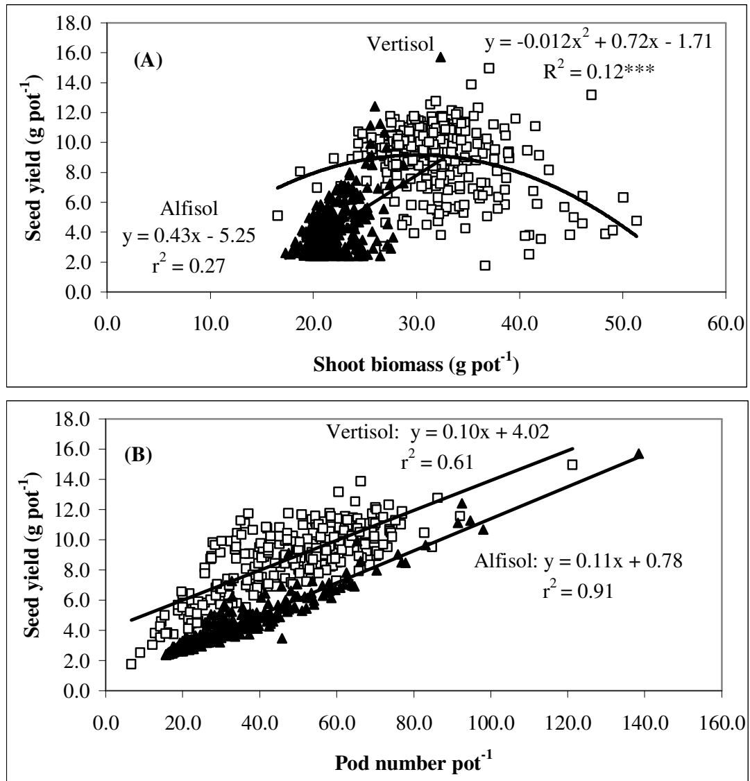
Fig. 2 The relationship of seed yield of genotypes under salinity with that of (A) shoot biomass under salinity and (B) pod number under salinity in a Vertisol soil in 2005-06 (open squares) and an Alfisol soil in 2007-08 (solid triangles).
