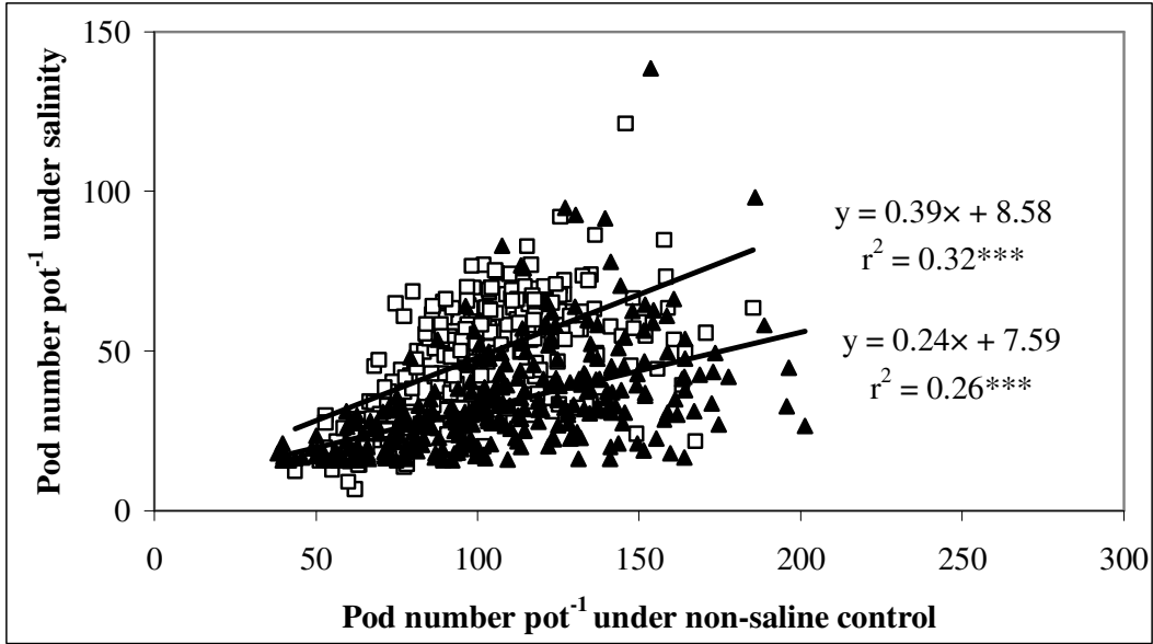
Fig. 5 The relationship between the pod numbers in the non-saline pots and in the saline pots in a Vertisol soil in 2005-06 (open squares) and an Alfisol soil in 2007-08 (solid triangles).
