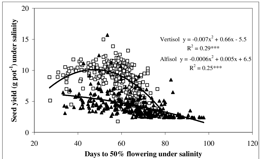
Fig. 1 The relationship between 50% flowering (days after sowing) and the seed yield under salinity in a Vertisol soil in 2005-06 (open squares) and an Alfisol soil in 2007-08 (solid triangles).
