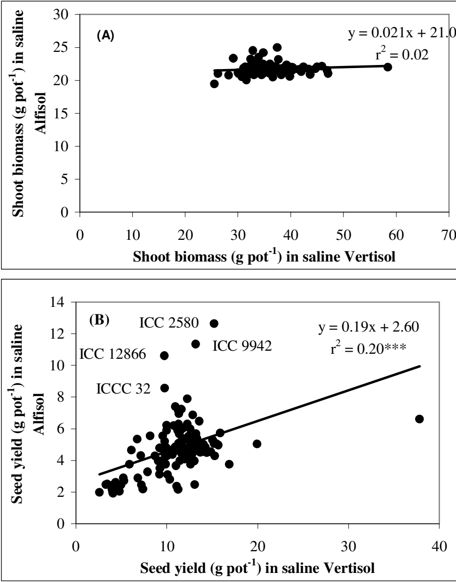
Fig. 4 The relationship of (A) shoot biomass production in the saline Alfisol soil with that of the saline Vertisol soil, and (B) the seed yield in the saline Alfisol soil with that in the saline Vertisol soil.
