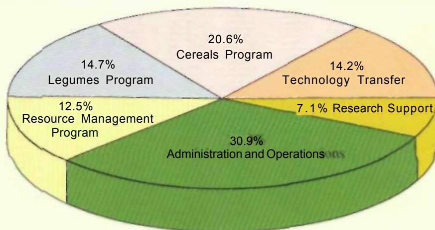
Figure 15. ICRISA T's resource allocations (core operations).
