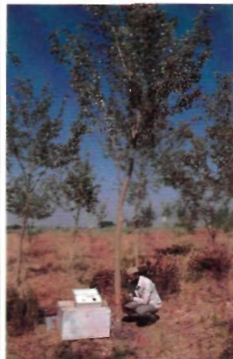
Transpiration is measured in trees using the heat pulse system.
