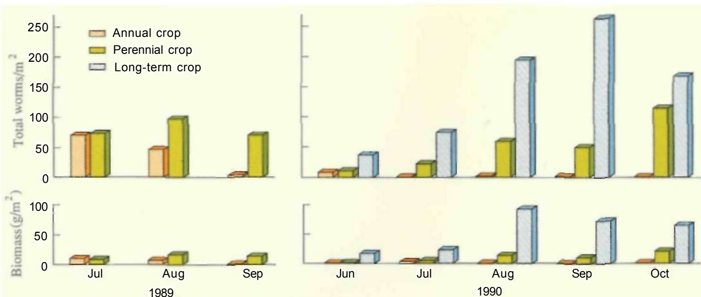
Figure 7. Temporal changes in earthworm population and biomass for three crop management systems on an Alfisol at ICRISAT Center during 1989 and 1990.
