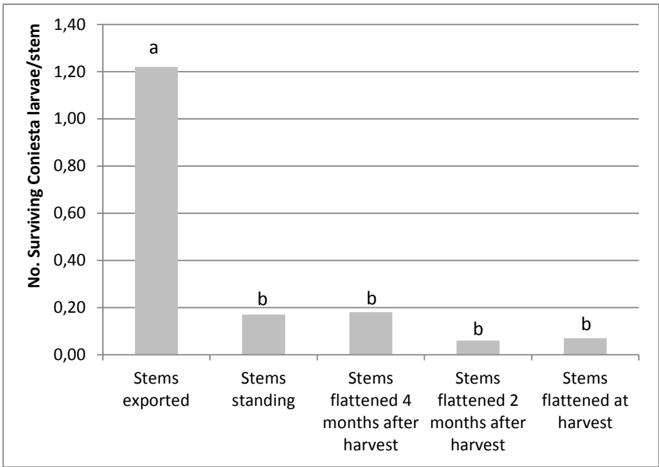
Fig. 1. MSB (Coniesta) survival in millet stems recorded at Sadore at the end of the dry season (May 2011)
