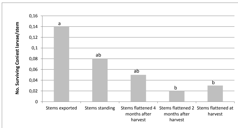
Fig. 2. MSB (Coniesta) survival in millet stems recorded at Doukoudoukou at the end of the dry season (May 2011)
