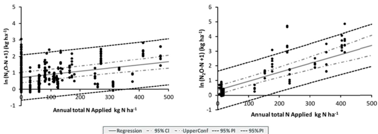
Fig. 3. The relationship between \text{N}_2\text{O} emissions and added N input (in the form of organic manures and synthetic N fertiliser) for (a) arable sites and (b) grassland sites. \ln(\text{N}_2\text{O}) ( \text{kg N}_2\text{O-N ha}^{-1} ). The data set includes multiple data points from each site.
