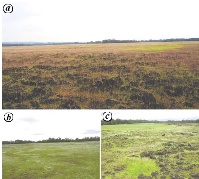
Figure 1. Manmanhara plateau views: a , During pre-monsoon. b, c , During monsoon.
