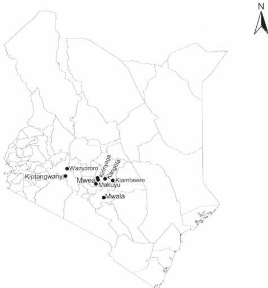
Figure 6-6: Distribution of PVS sites in eastern, central and western Kenya.
