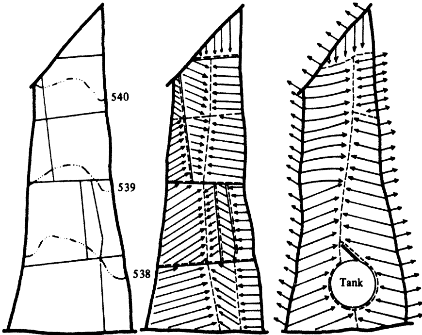
b. Broad bed and furrow system at 0.6% within field boundaries.
