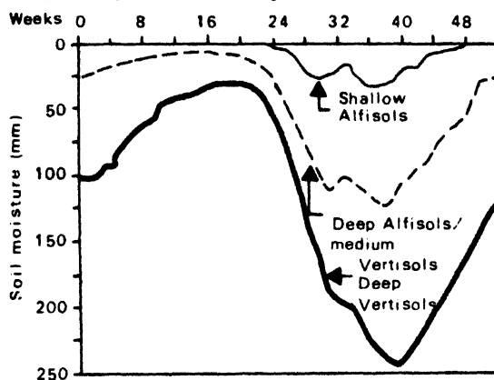
Fig. 3 Weekly soil moisture storage in three soils (Hyderabad, 1901–1970).
