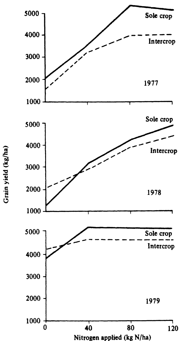
Fig. 2 Response of sole and intercropped rainy season sorghum to nitrogen on Vertisols at ICRISAT Center, 1977-79.
