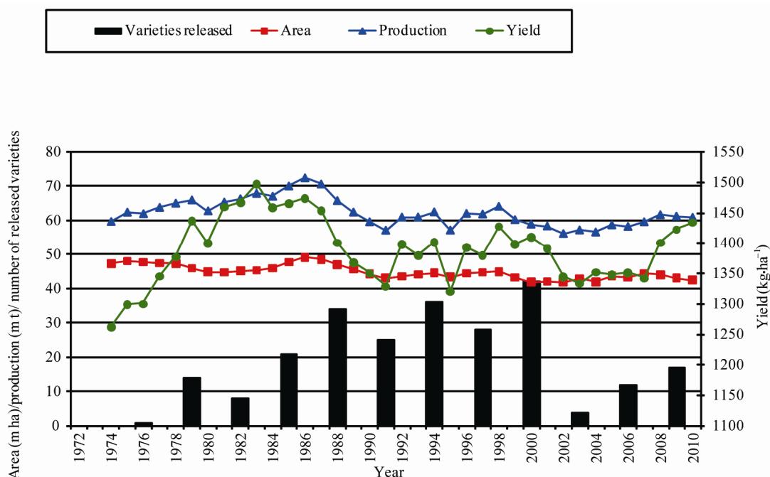
Figure 1. Three-year moving average for sorghum area, production, yield; and number of released varieties (3-years total) based on ICRISAT-bred material globally.
