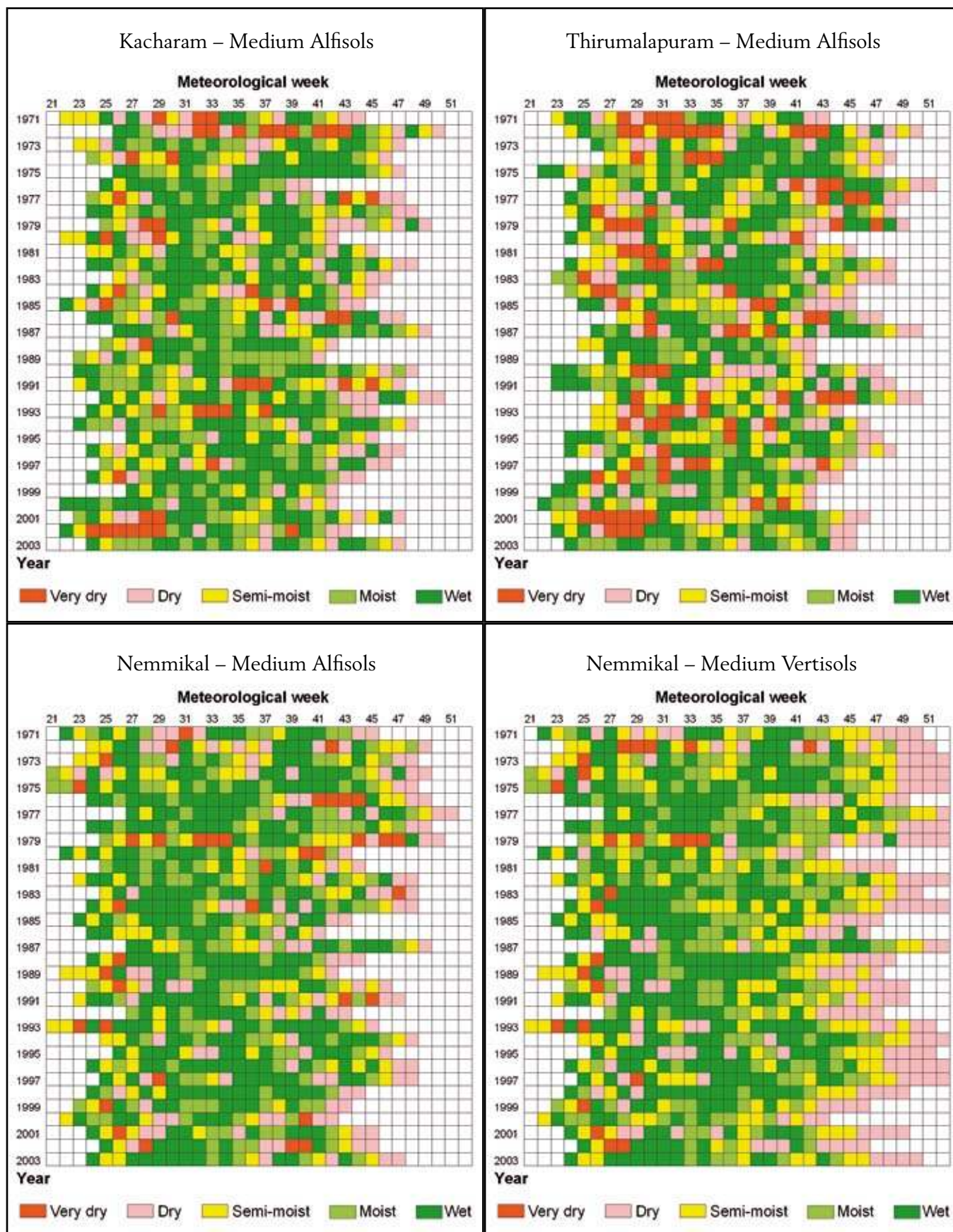
Figure 14. LGP, dry and wet spells at watershed locations.
