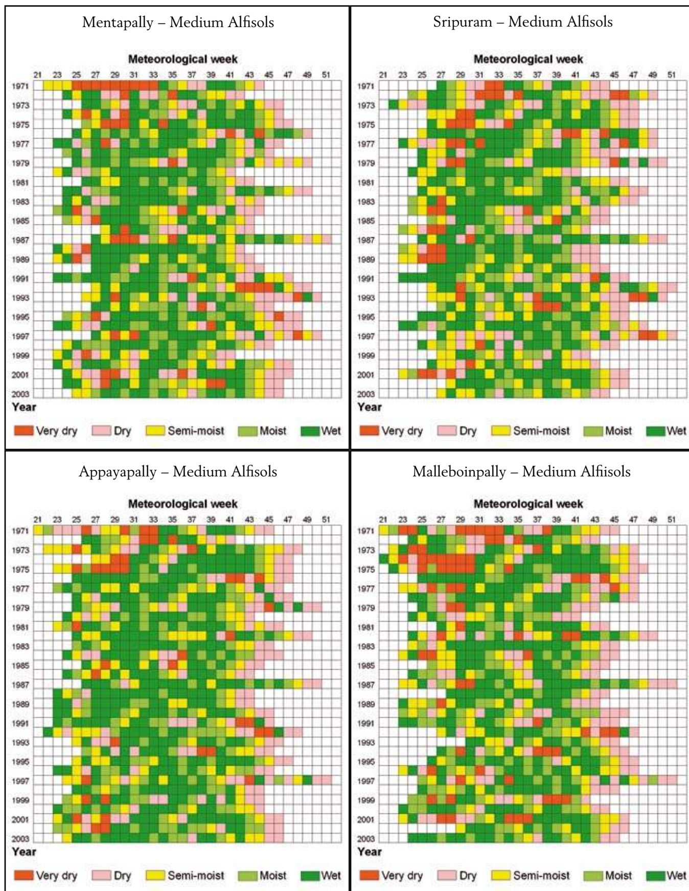
Figure 15. LGP, dry and wet spells at watershed locations.
