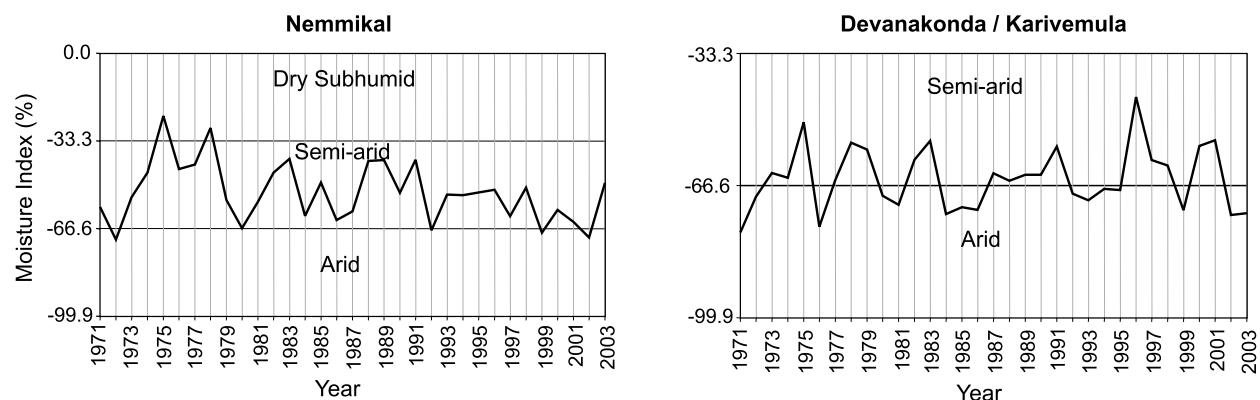
Figure 7. Climatic variability at Nemmikal and Devanakonda/Karivemula.
