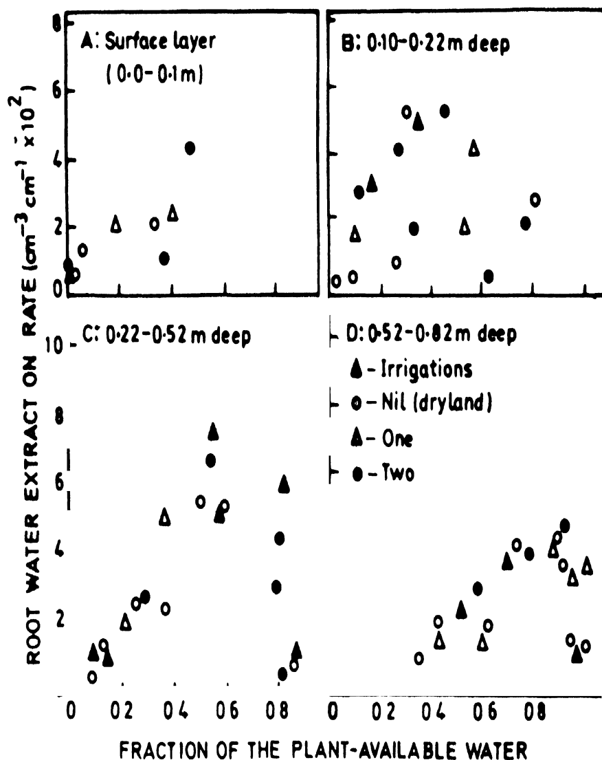
Figure 7 Effect of the fraction of plant-available water on water-extraction rates in four soil layers of a Vertisol by roots of twice irrigated and dryland sorghum crops. (Lines are fitted by hand). CSH 8R, Vertisol, ICRISAT Center (Unpublished data of Sardar Singh)
