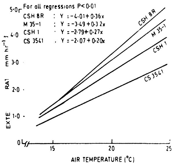
Figure 5 Effect of air temperature on leaf-extension rates of four sorghums genotypes. All regressions are significant at P < 0.01 (Unpublished data of N Seetharama)
