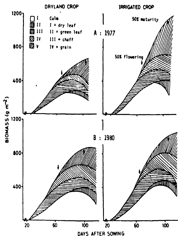
Figure 6 Seasonal changes in dry matter in various plant parts of rabi sorghum grown under dryland and irrigated conditions. The soil water profile was fully charged in 1980, but only 77% charged at sowing in 1977. CSH 8R, Vertisol, ICRISAT Center (Unpublished data of Sardar Singh and N. Seetharama)
