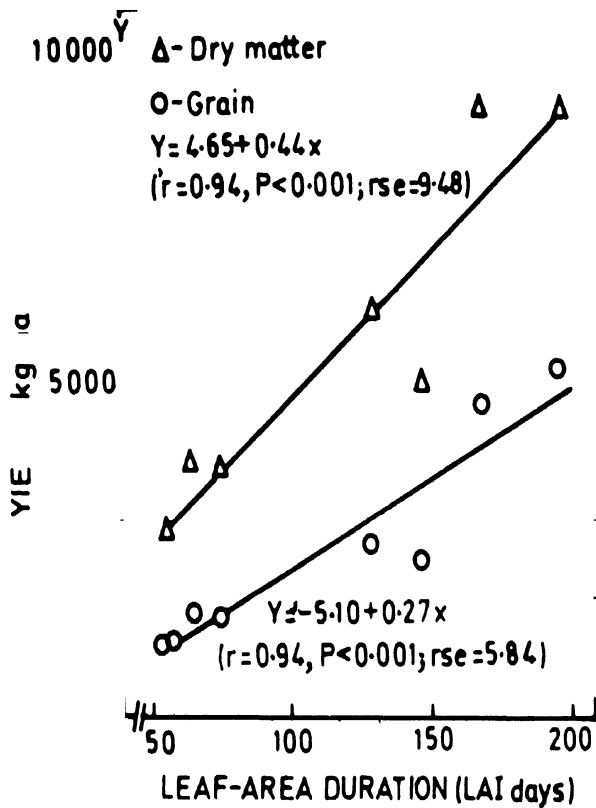
Figure 4 Relationships between leaf-area duration (LAI days) and grain, and total dry matter yields. ICRIAT Center, rabi 1981
