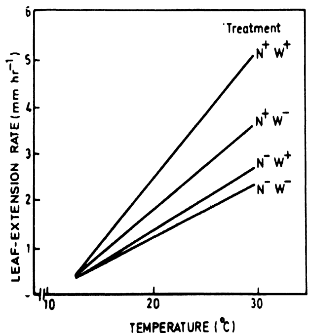
Figure 3 Relationships between air temperature and leaf-extension rates (LER). All linear regressions are highly significant ( P < 0.01 ). ICRISAT Center, rabi 1981 (Based on Seetharama et al. 1982b)
