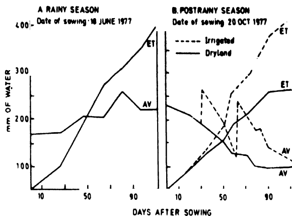
Figure 1 Seasonal trends in evapotranspiration (ET), and available-profile water (AV) for kharif (A), and rabi season (B) sorghum grown on a deep Vertisol, ICRISAT Center, 1977 (unpublished data of Sardar Singh)
