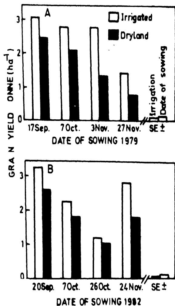
Figure 2 Grain-yield response of sorghum (mean of 5 cultivars) to irrigation and date of sowing during rabi in 1979 (A) and 1982 (B). Sorghum hybrid CSH 8R was sown on four dates on a deep Vertisol from September to November in 1979, and 1982. Irrigated treatments received two irrigations during each year before flowering, each time to fully recharge the soil profile. Vertisol, ICRISAT Center (Based on Reddy et al. 1987)
