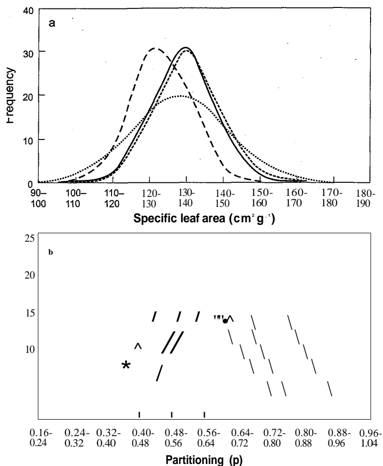
Figure 7. Specific leaf area (SLA) (a) and partitioning, P (b) in 64 groundnut germplasm accessions of different botanical types. Postrainy season 1992, ICRISAT Center (Spanish-^, Valencia____, Virginia bunch...., Virginia runner-----). (Source: Nageswara Rao et al., 1994).
