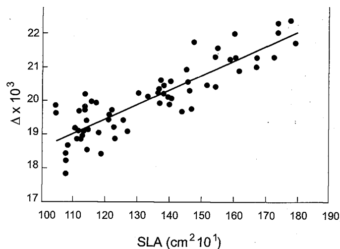
Figure 6. Relationship between the mean SLA and p in leaves of four groundnut cultivars under the two drought treatments, p = 14.2 + 0.04 \text{ SLA} , ( r^2 = 0.81 , P < 0.01 ). (Source: Wright et al., 1994)
