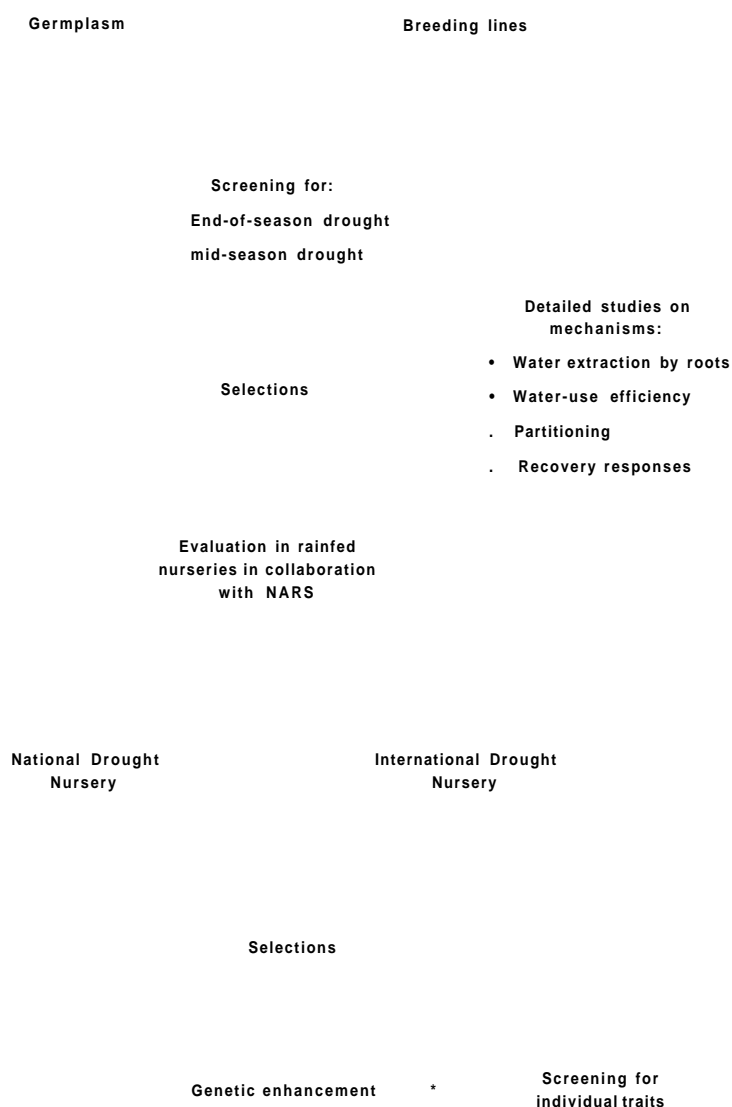
Figure 4. Flow of groundnut genotypes in drought screening programme at ICRISAT.
