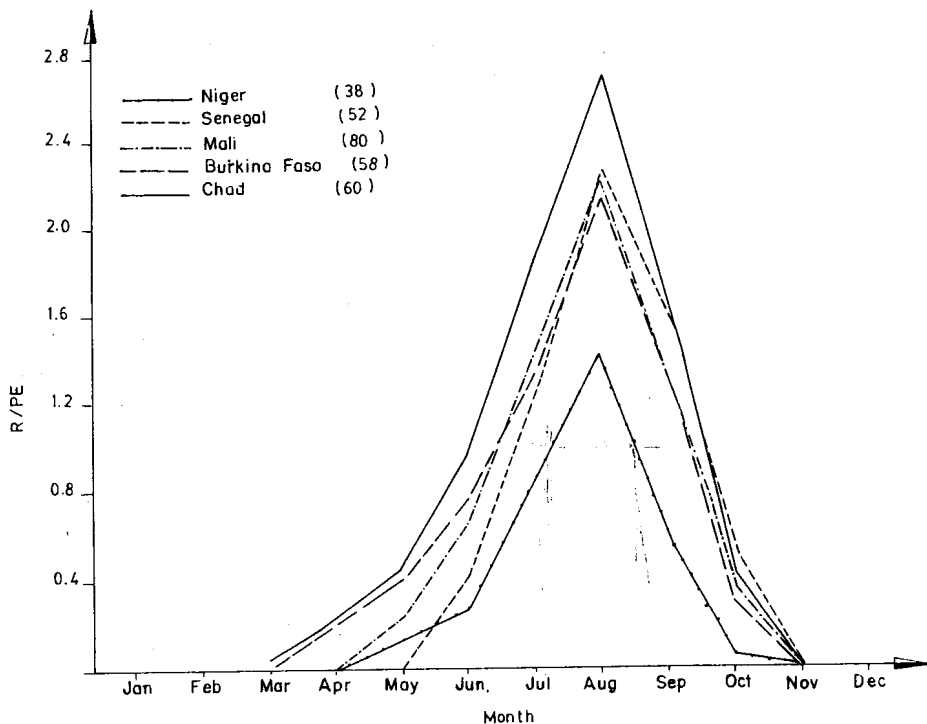
Fig. 1. Seasonal progression of R/PE [rainfall/potential (reference) crop evaporation] in five West African countries (number of stations over which R/PE was computed is given in parentheses).
