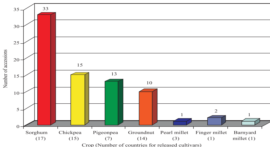
Figure 1. Number of accessions released as varieties worldwide from the basic germplasm supplied from ICRISAT genebank during 1976-2008.
