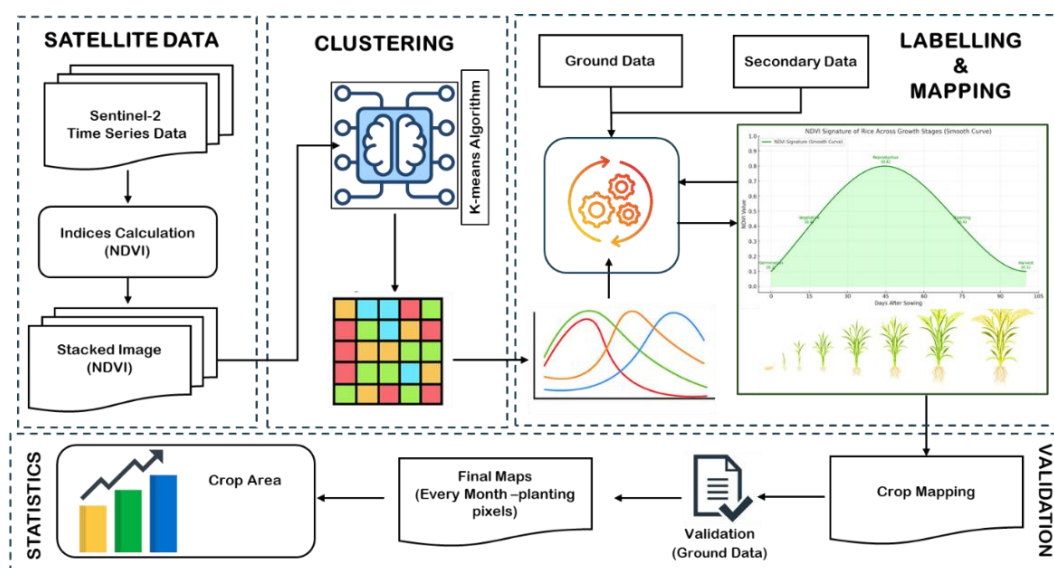
Figure 3: Methodology for crop classification
