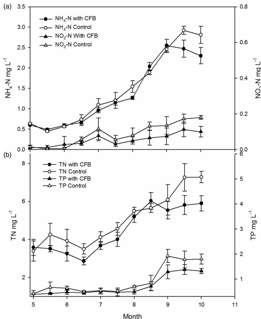
Figure 3 | Seasonal variation of inorganic nutrients during the culture phase in ponds with CFB and control. Error bars represent \pm SD.
