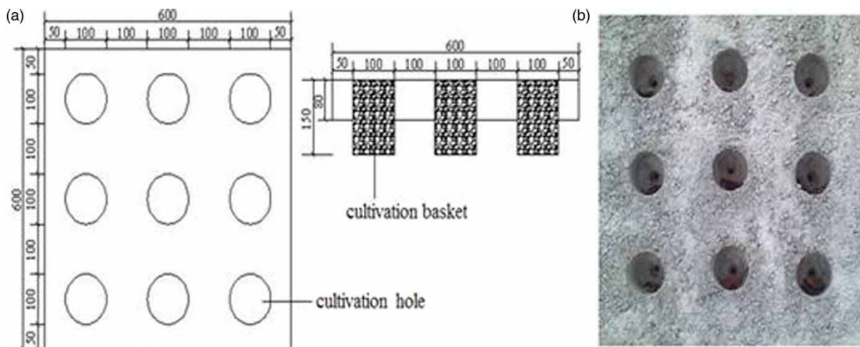
Figure 1 | Schematic diagram showing design and dimensions of CFB (a) and molded ceramsite plate with cultivation hole (b).
